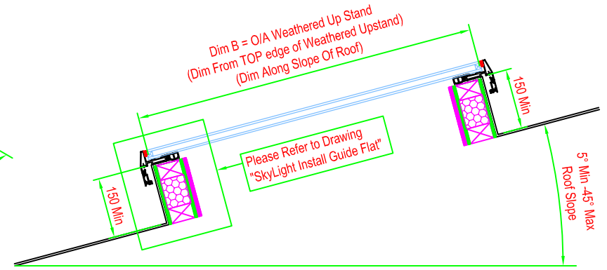
Section B-B (For Sloping Roof)
