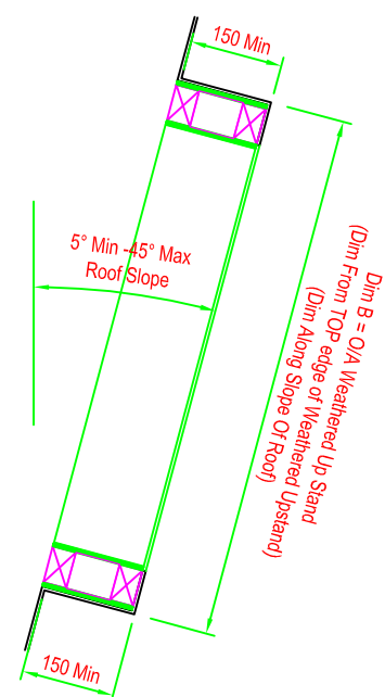
Section B-B (For Sloping Roof)
